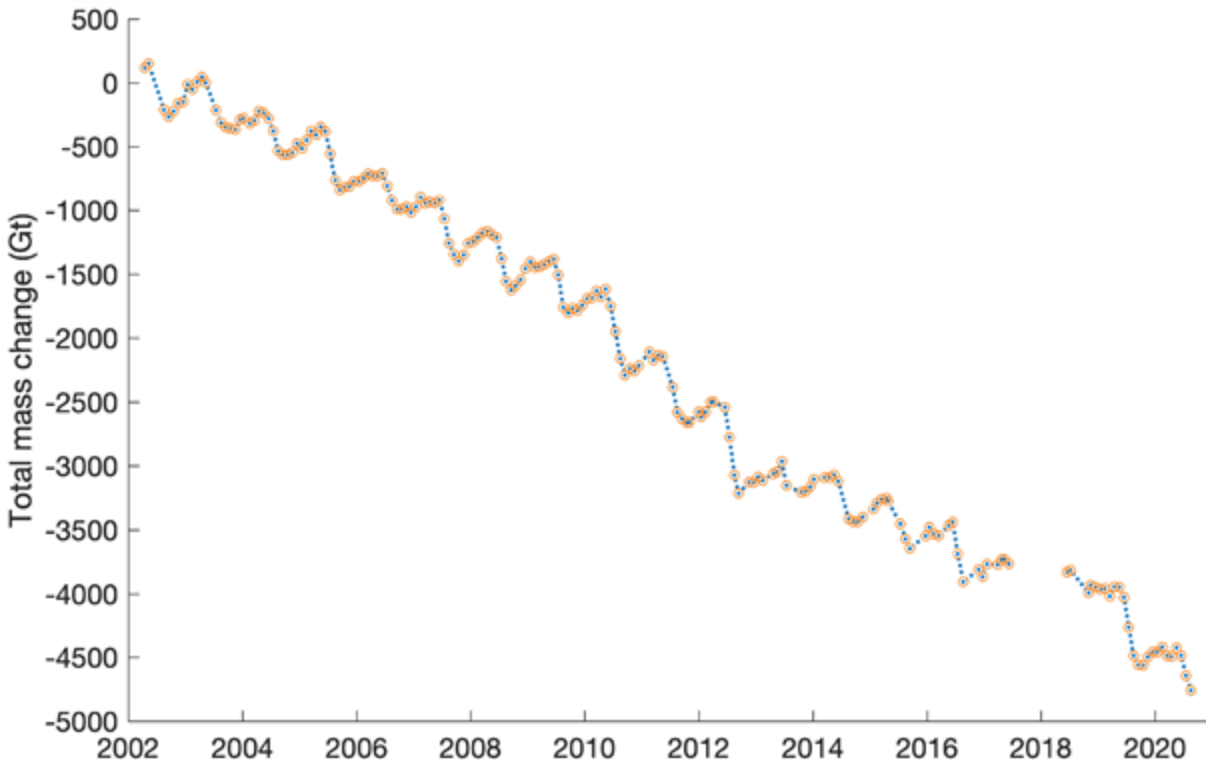
Fig. 5. Total mass change (Gt) of the Greenland ice sheet from April 2002 to August 2020 determined from GRACE (2002–2017) and GRACE-FO (2018–Present). An averaging kernel (Wahr et al. 1998) is applied to the JPL RL06 Level 2 monthly spherical harmonic solutions after the applied corrections: Geocenter (Sun et al. 2016; https://podaac-tools.jpl.nasa.gov/drive/files/allData/grace/docs/TN-13_GEOC_JPL_RL06.txt ); C_{20} and C_{30} (Loomis et al. 2019b, 2020; https://podaac-tools.jpl.nasa.gov/drive/files/allData/gracefo/docs/TN-14_C30_C20_GSFC_SLR.txt ); and glacial isostatic adjustment (Peltier et al. 2018; ICE-6G_D). The applied averaging kernel has been tuned to match the trends observed by the NASA GSFC mascons (Loomis et al. 2019a), which was designed to mitigate leakage of other nearby mass change signals into the Greenland ice sheet estimates.
