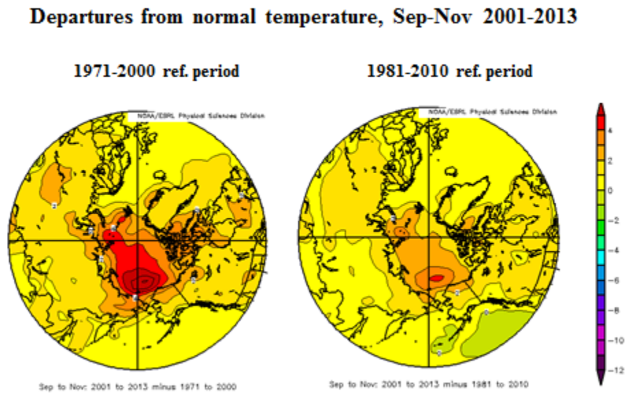
Fig. 10.4. Departures of autumn (September-November) air temperatures for 2001-2013 from the means of the 30-year reference periods (a, left) 1971-2000 and (b, right) 1981-2010.
